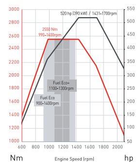
DE13 - 520 hp
