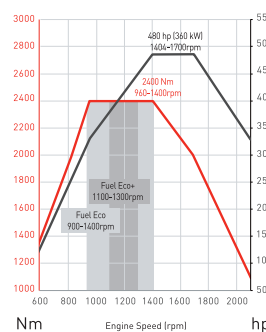
DE13 - 480 hp
