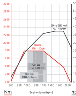
DE11 - 380 hp
