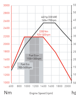
DE13 - 440 hp
