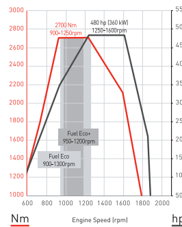
DE13 TC - 480 hp
