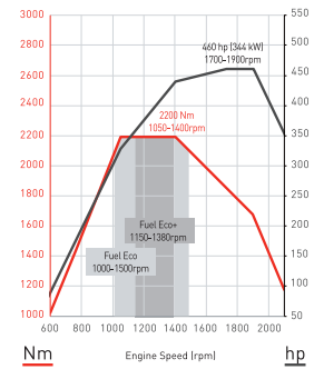
DE11 - 460 hp
