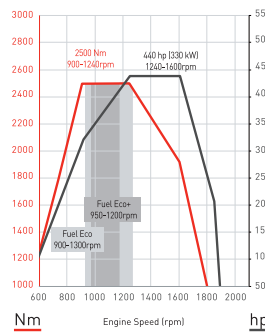
DE13 TC - 440 hp
